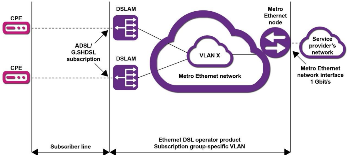
Figure 3: Ethernet DSL operator product, access-group-specific VLAN and a subscriber line
