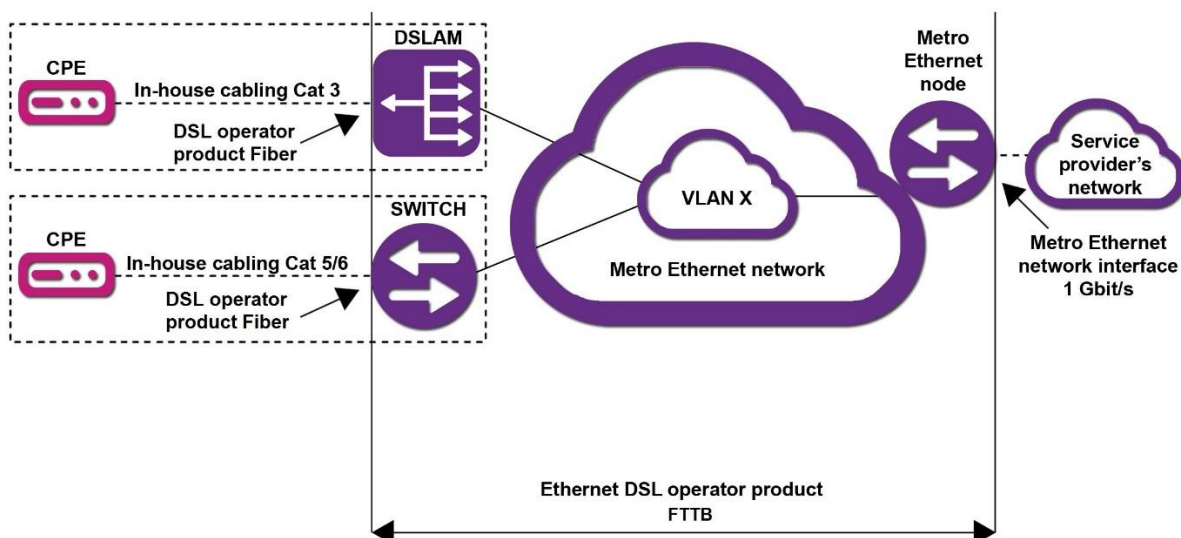
Figure 1: DSL operator product Fiber.
