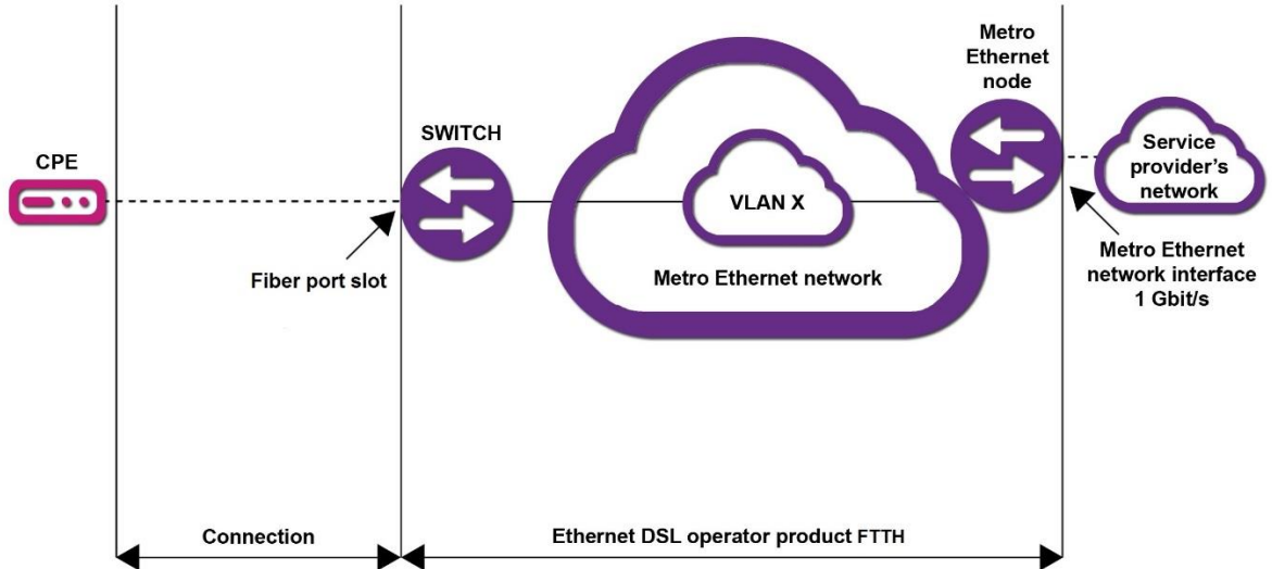
Figure 2: DSL operator product Fiber port slot and connection.
