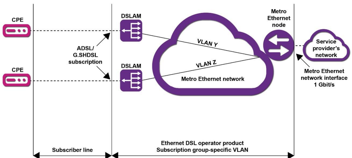
Figure 4: Ethernet DSL operator product, access-specific VLAN and a subscriber line
