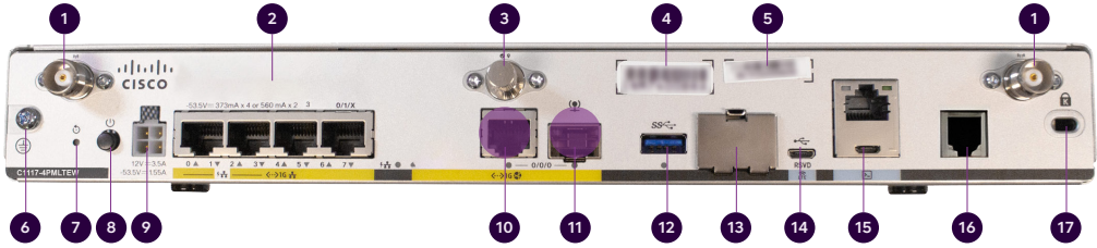
Figure 7: Cisco C1117-4PMLTEW rear connections
