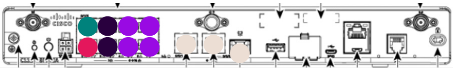
Figure 8. Router port designations for a 5G implementation
