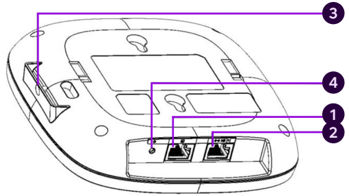
Figure 13. Cisco C9105AXI-E
